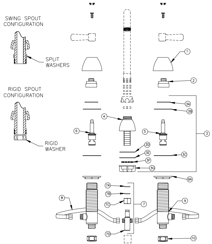
Z831A1-XL PICTURED
