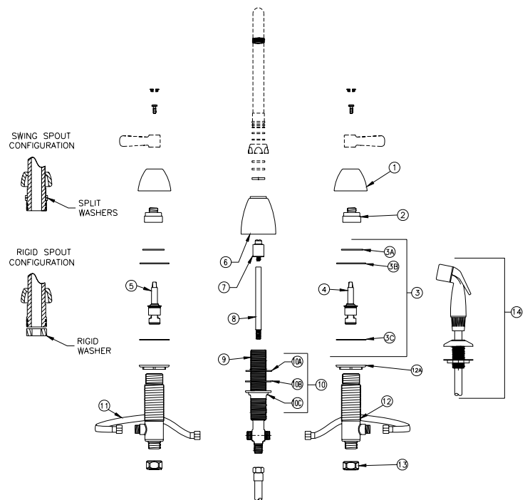
Z831A1-XL-HS PICTURED
