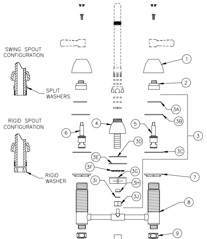
Z831A1-XL-ICT PICTURED
