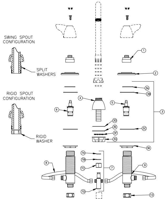
Z831A1-XL-HS PICTURED
